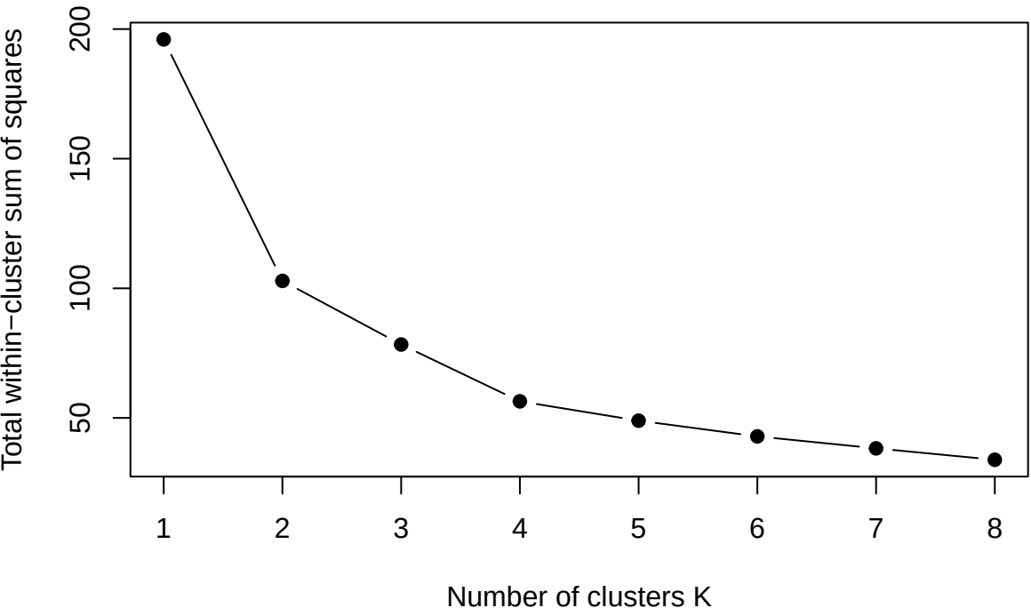
USArrests: K-means elbow plot
